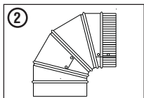
90° Adjustable Elbow
